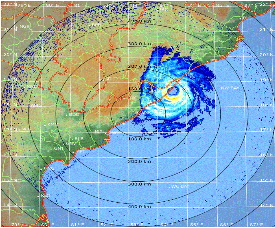
PPI (dBZ) 23:00 / 10-Oct-2018 Visakhapatnam
