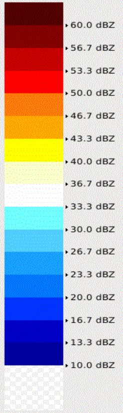
PPI (dBZ) 23:00 / 10-Oct-2018 Visakhapatnam
